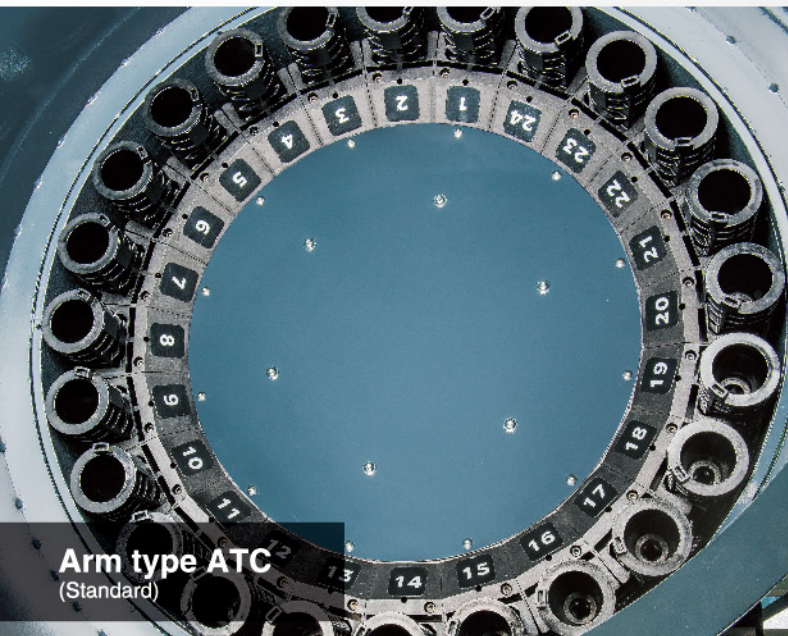
Magazine With Full Cover For CE Specification.
